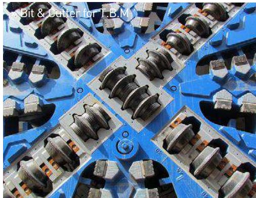
» Bit & Cutter for T.B.M
