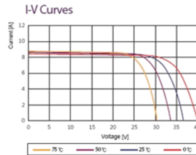
IV behaviour for various temperatures
