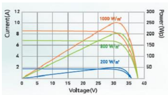
IV behavior at various degrees of irradiation intensity
